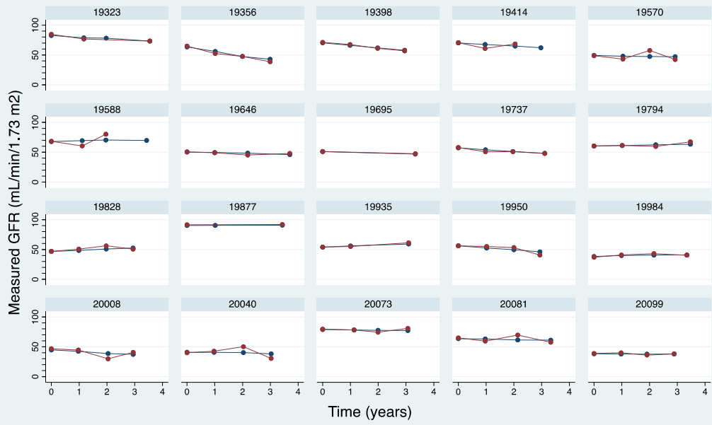
Observed and fitted values from the random coefficients covariate model Graphs by participant
